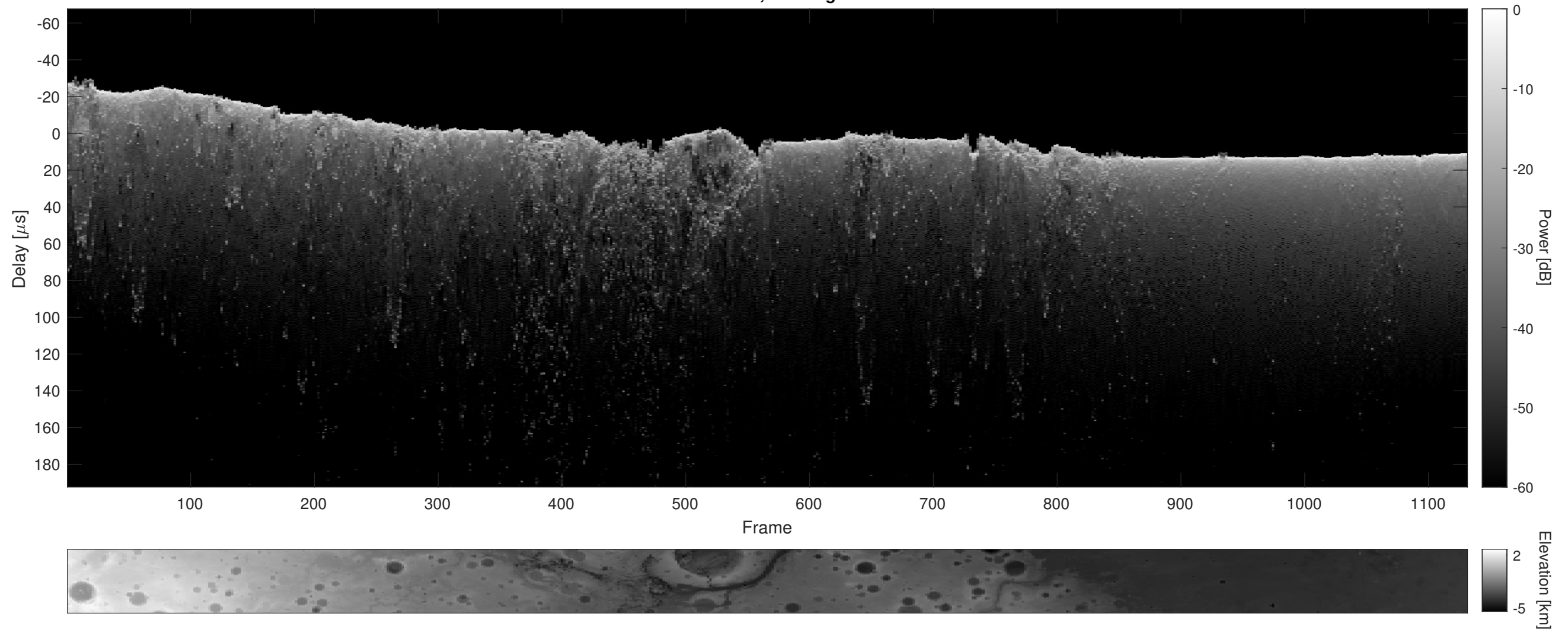
Orbit 18645, Cluttergram
