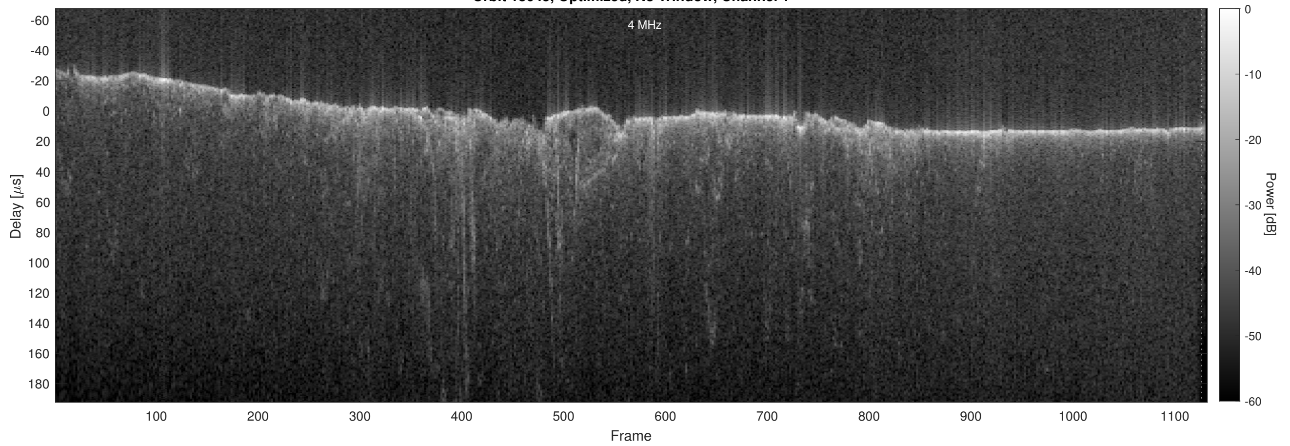
Orbit 18645, Optimized, No Window, Channel 2
