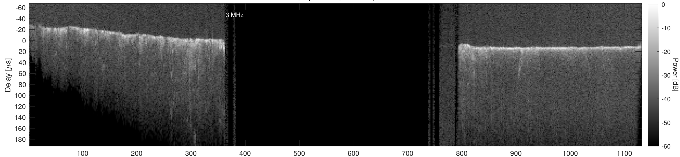
Orbit 18645, Cluttergram
