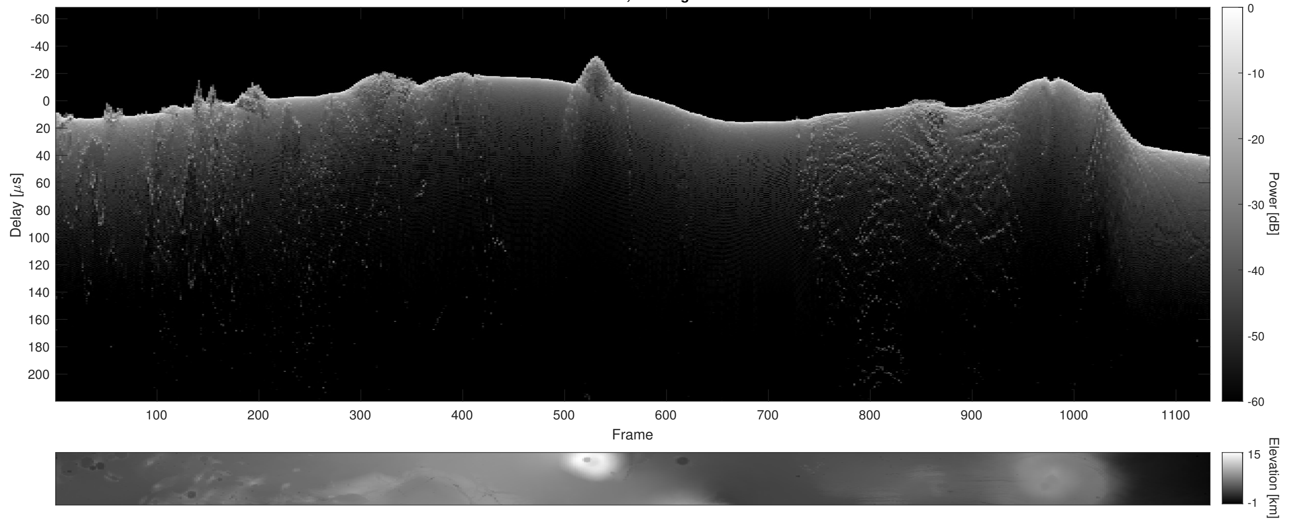
Orbit 18660, Cluttergram
