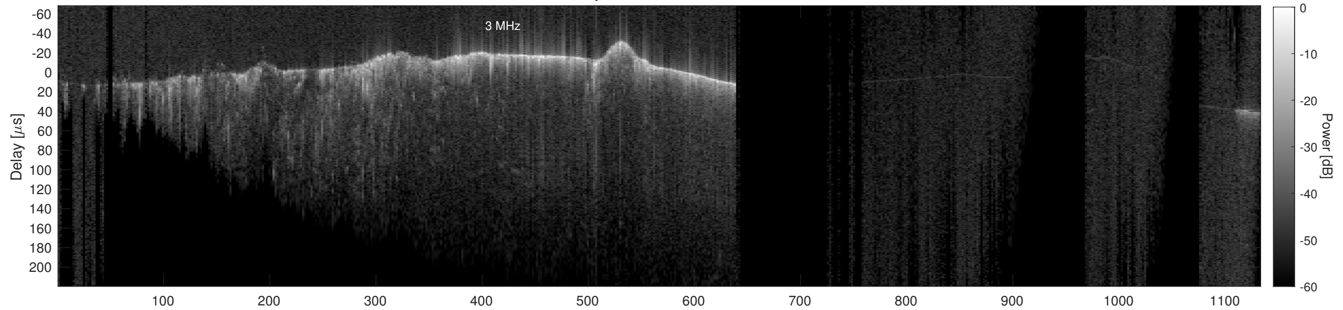
Orbit 18660, Cluttergram
