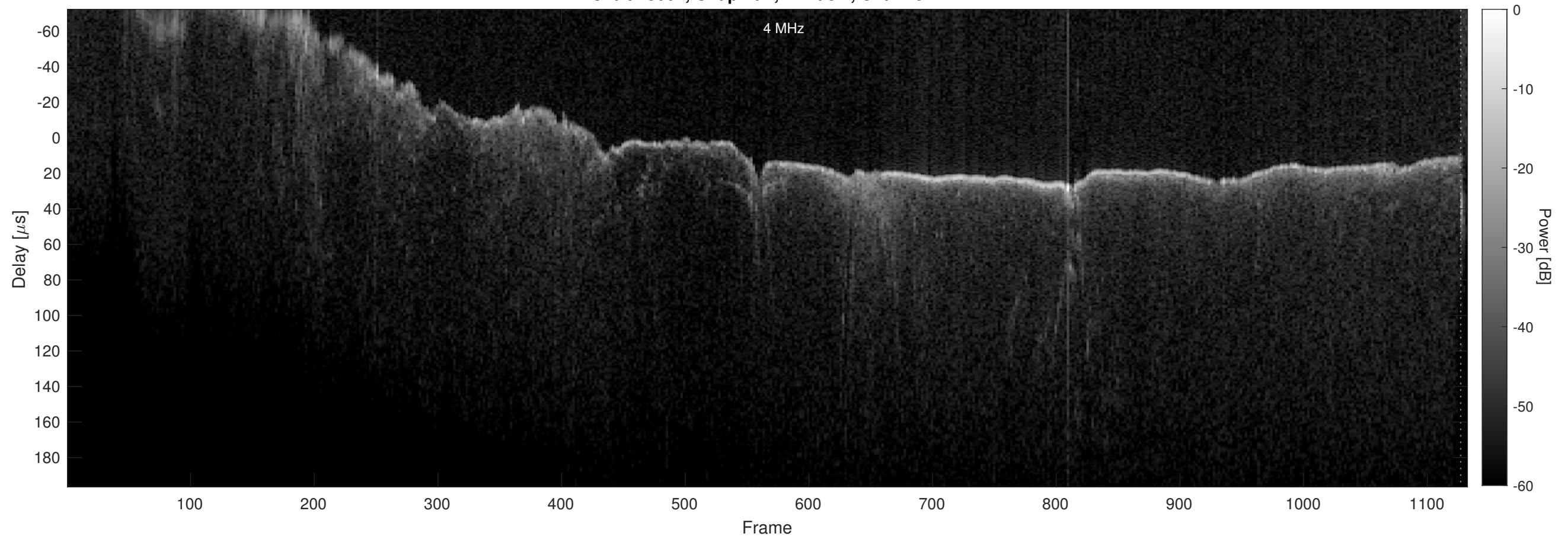
Orbit 18664, Chapman, Window, Channel 2
