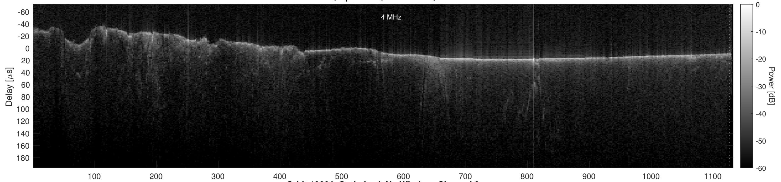
Orbit 18664, Optimized, No Window, Channel 2
