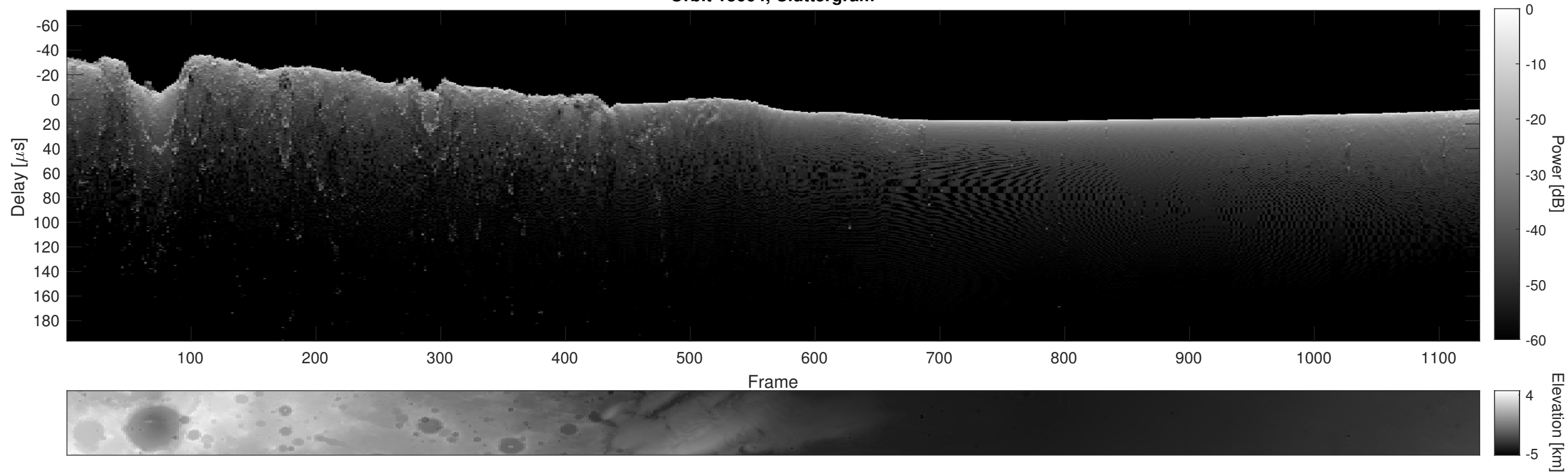
Orbit 18664, Cluttergram
