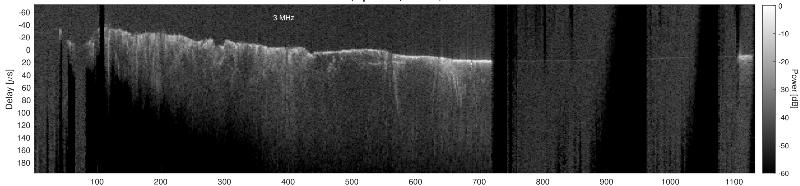
Orbit 18664, Cluttergram
