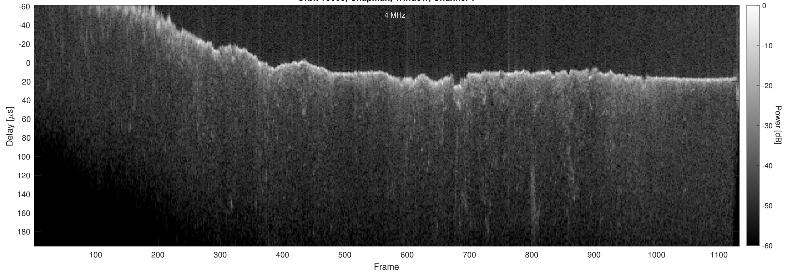
Orbit 18666, Chapman, Window, Channel 2
