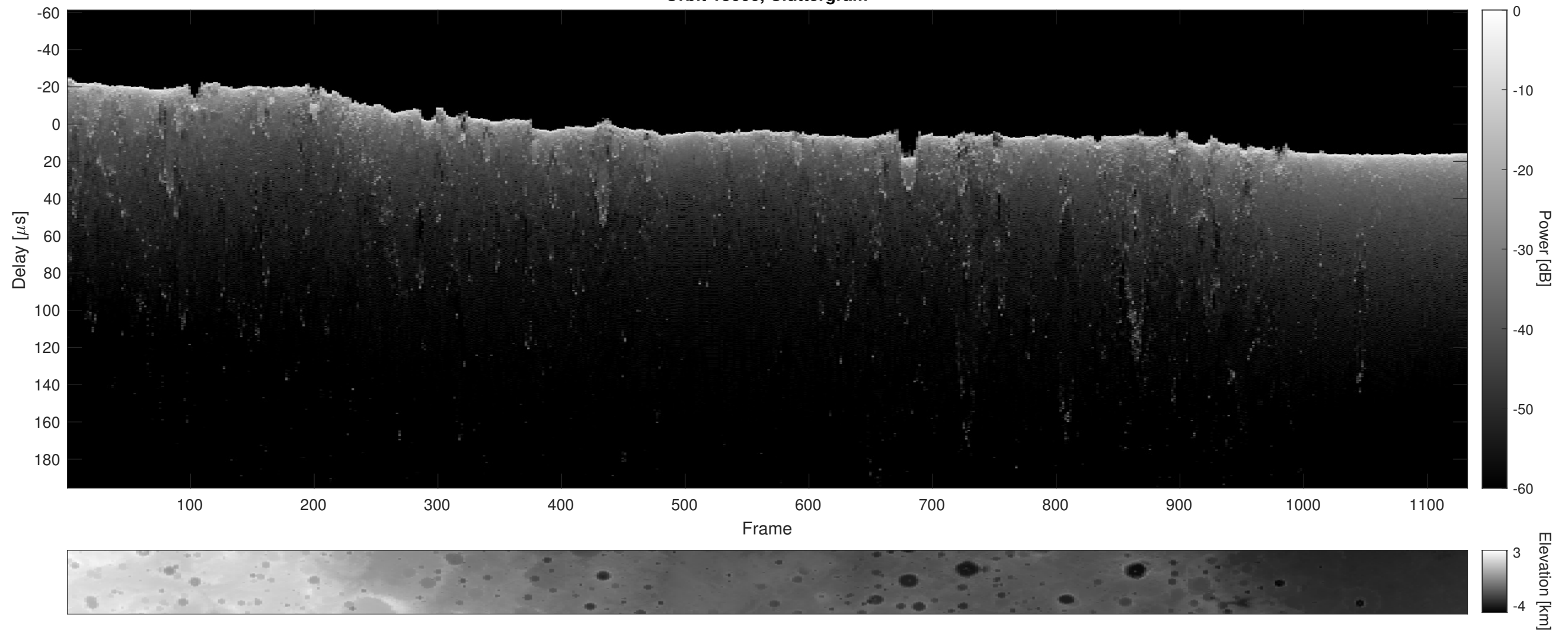
Orbit 18666, Cluttergram
