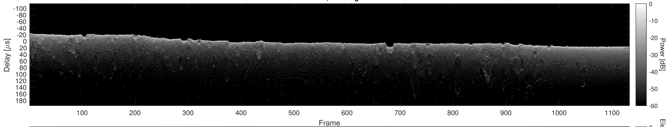
Orbit 18666, Cluttergram
