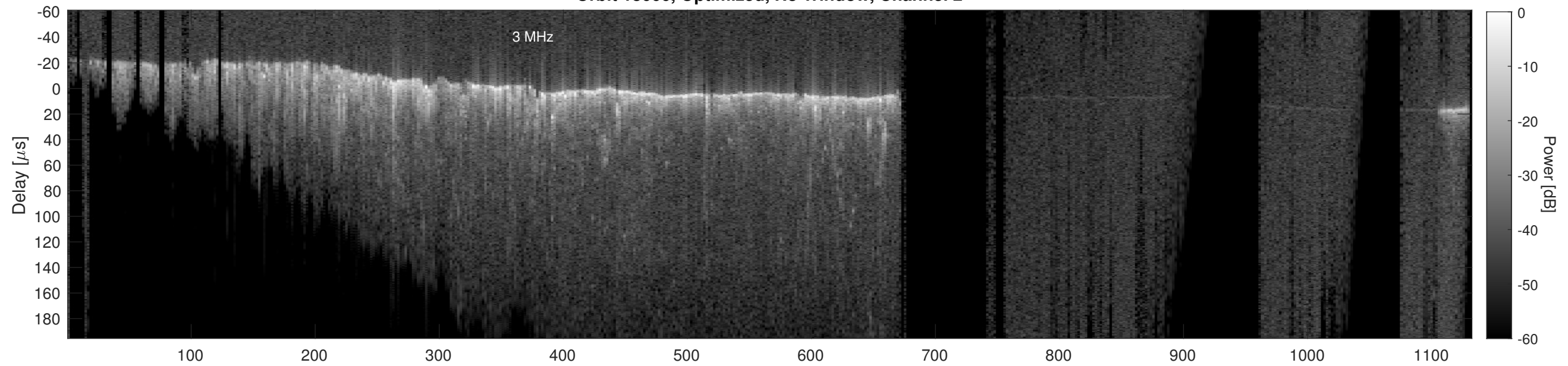
Orbit 18666, Cluttergram
