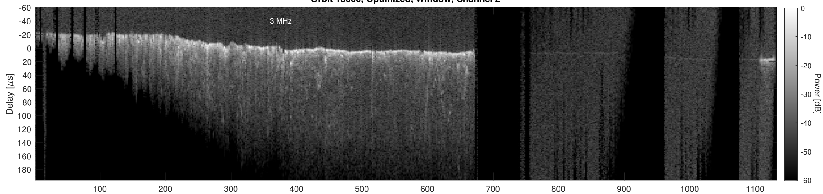
Orbit 18666, Cluttergram
