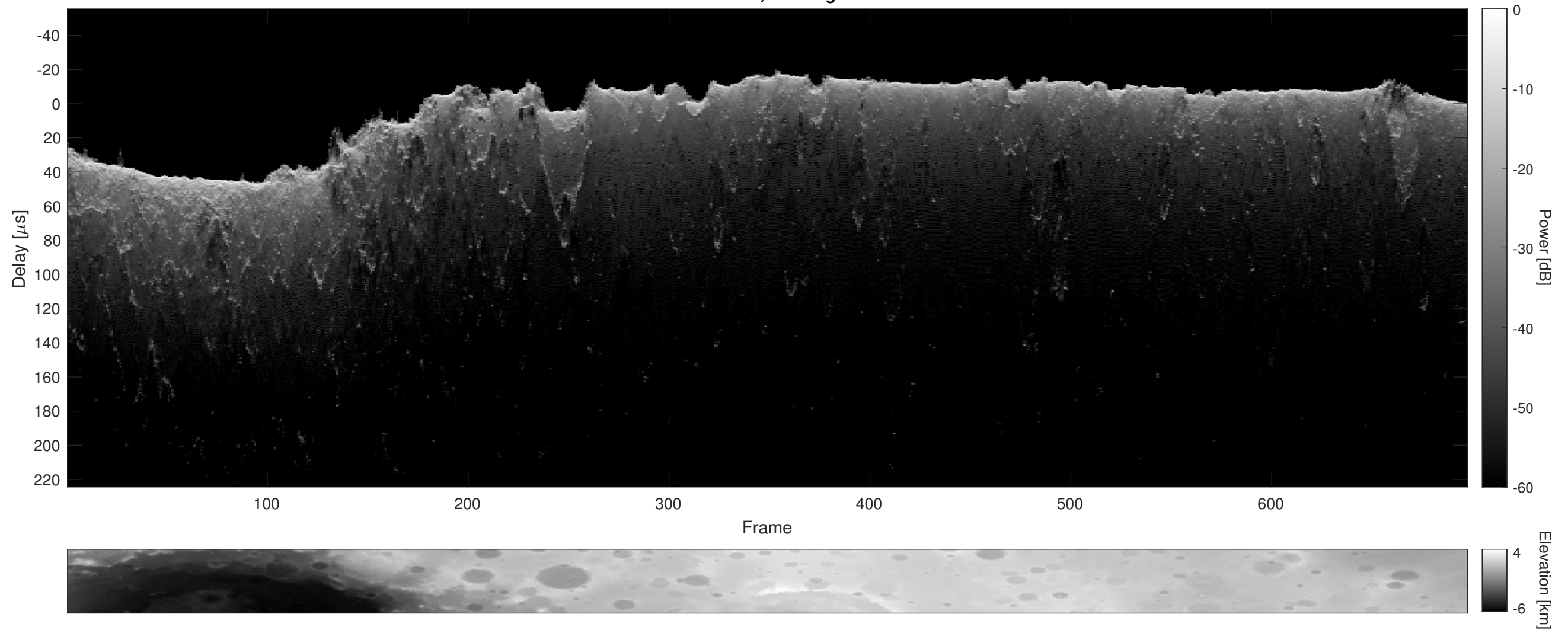
Orbit 18669, Cluttergram
