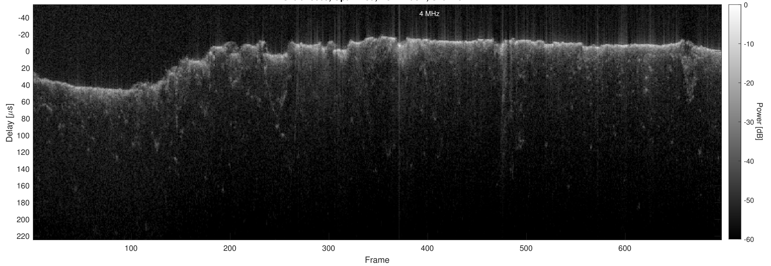
Orbit 18669, Optimized, No Window, Channel 2
