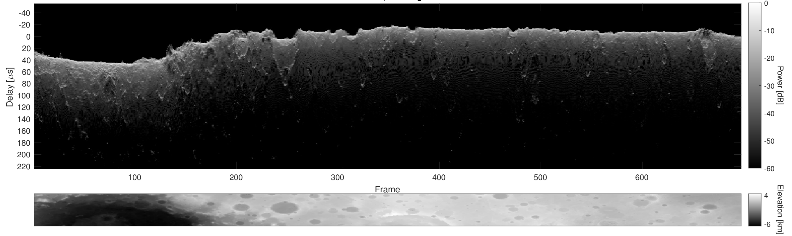
Orbit 18669, Cluttergram
