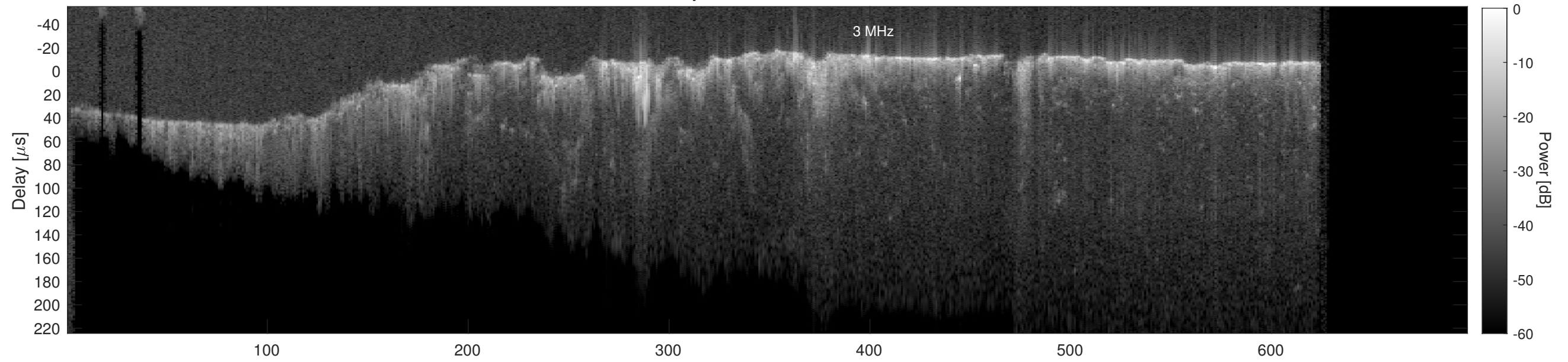
Orbit 18669, Cluttergram
