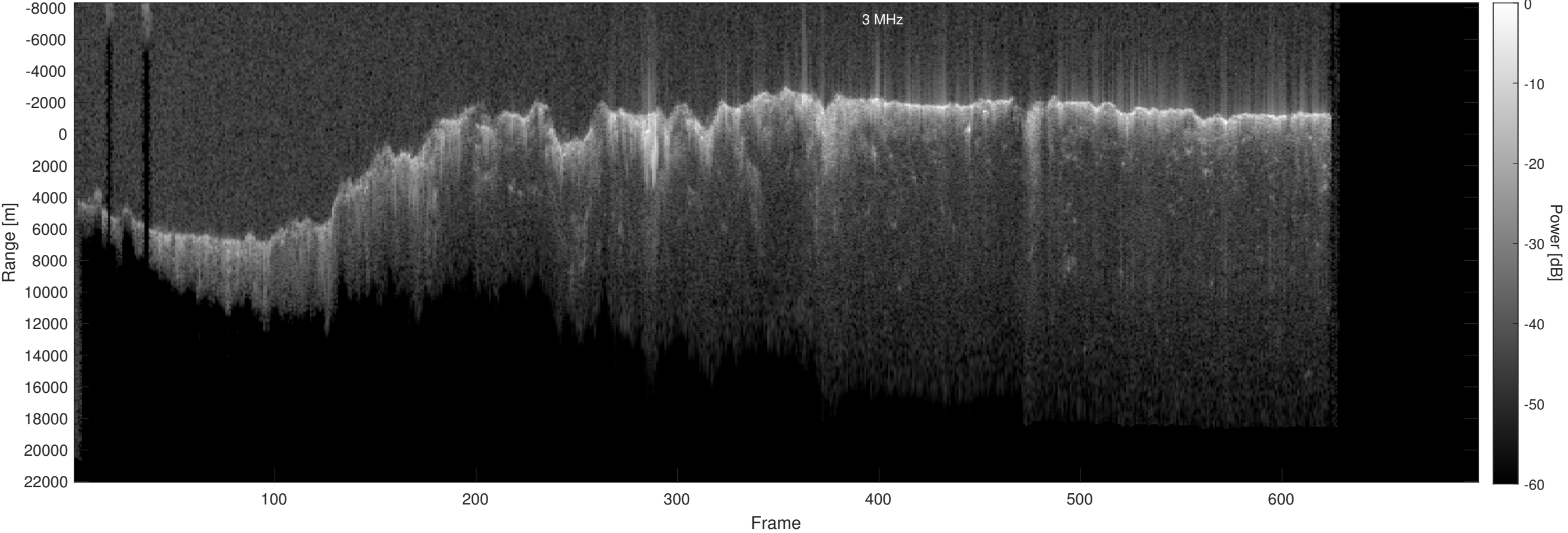
Orbit 18669, Optimized, No Window, Depth-Corrected, Channel 2
