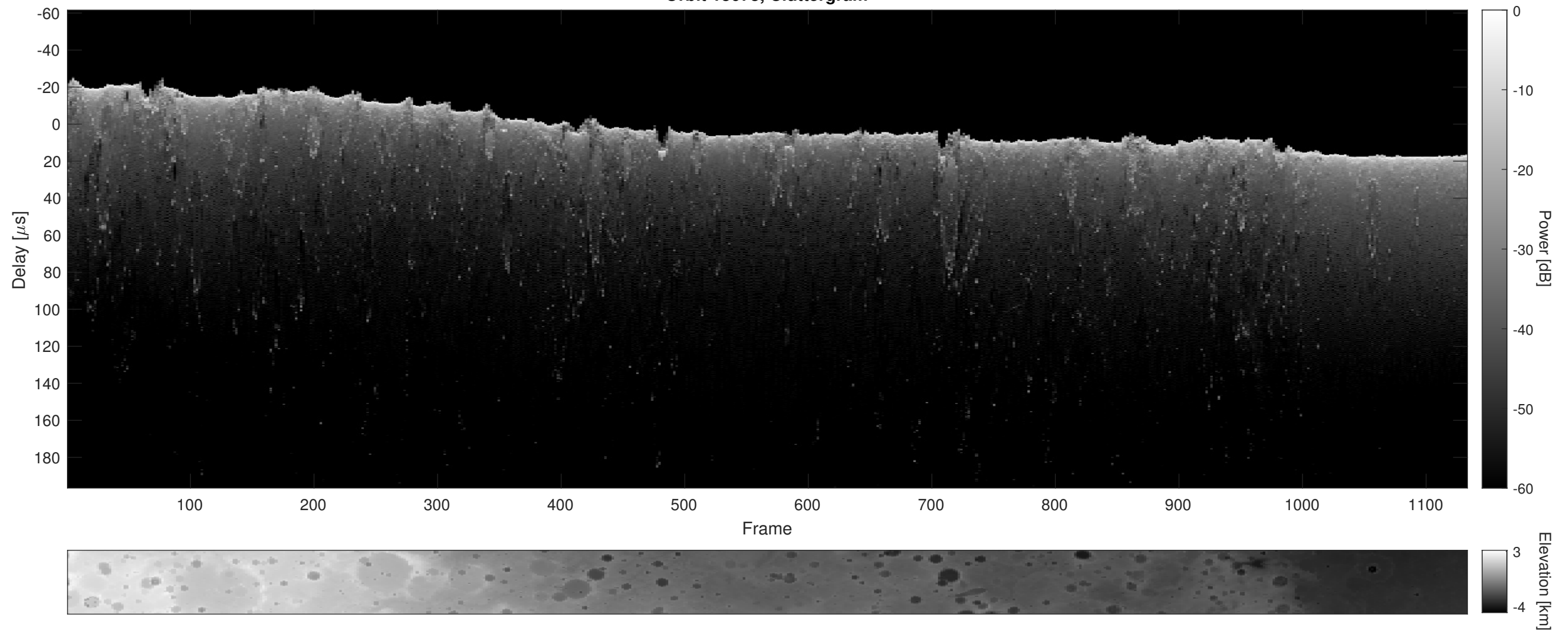
Orbit 18673, Cluttergram
