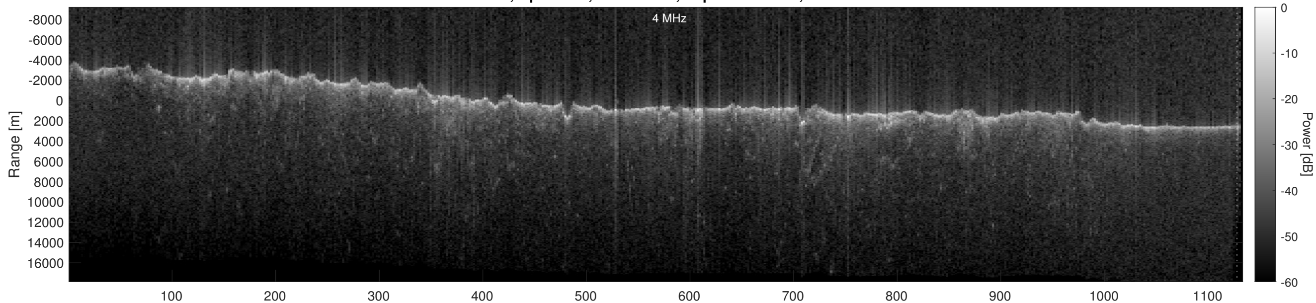
Orbit 18673, Optimized, No Window, Depth-Corrected, Channel 2
