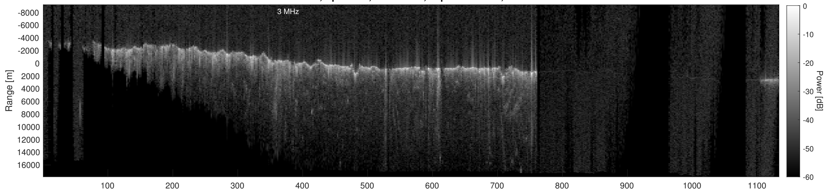
Orbit 18673, Depth-Corrected Cluttergram
