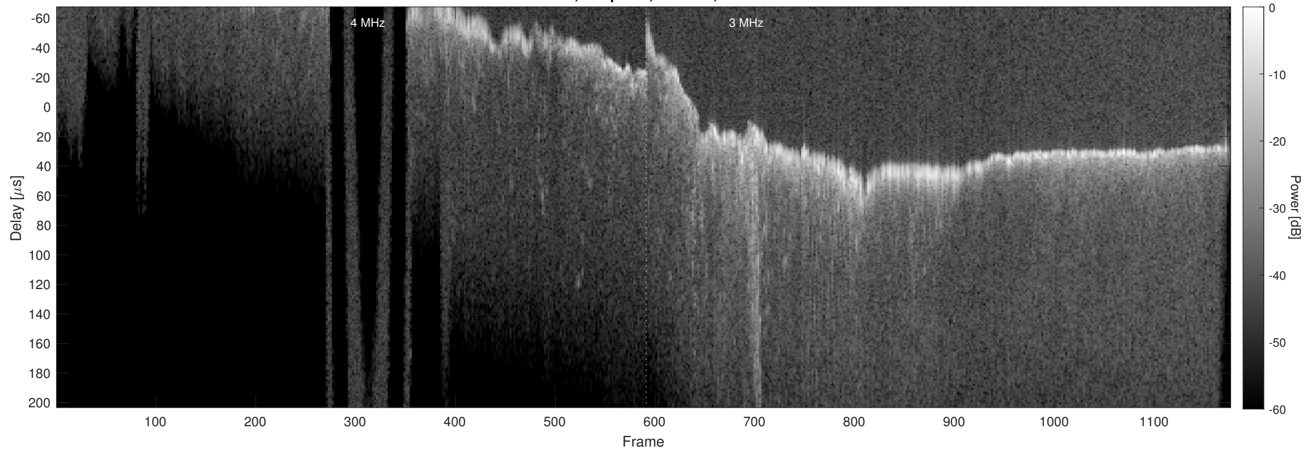
Orbit 18700, Chapman, Window, Channel 2
