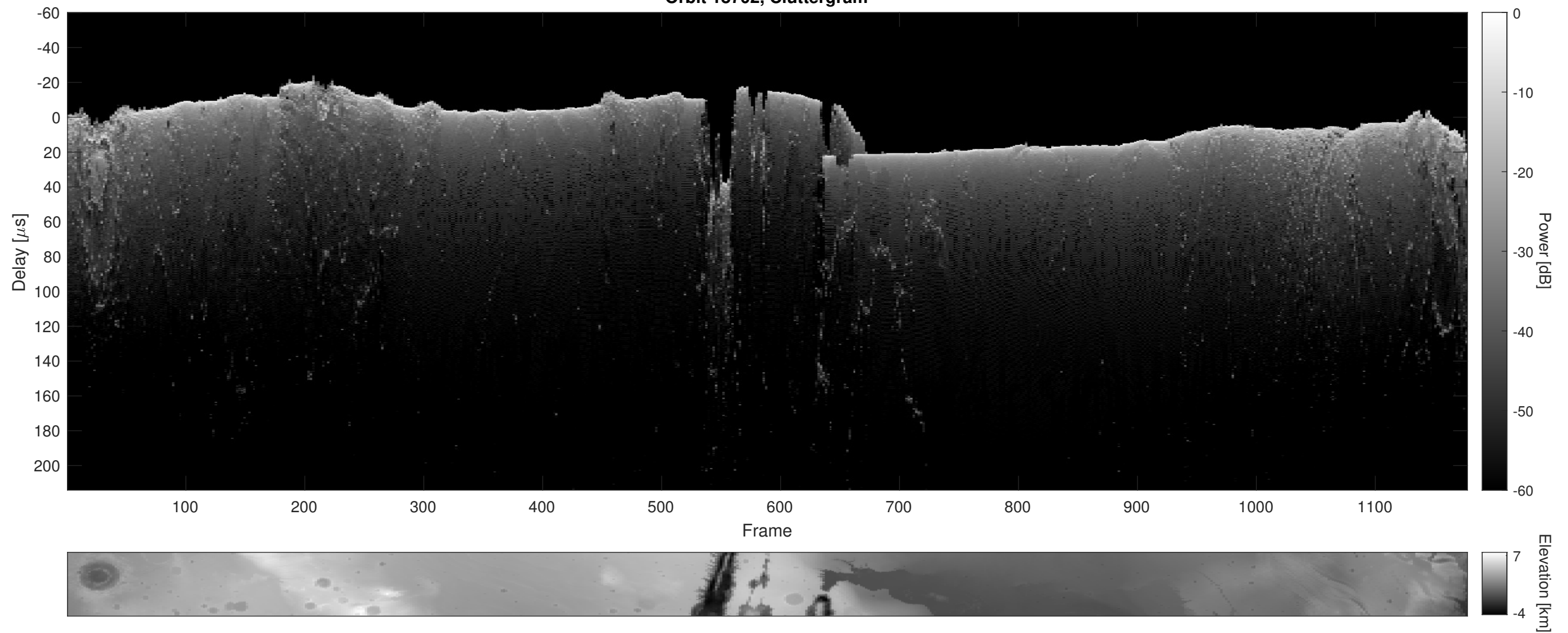
Orbit 18702, Cluttergram
