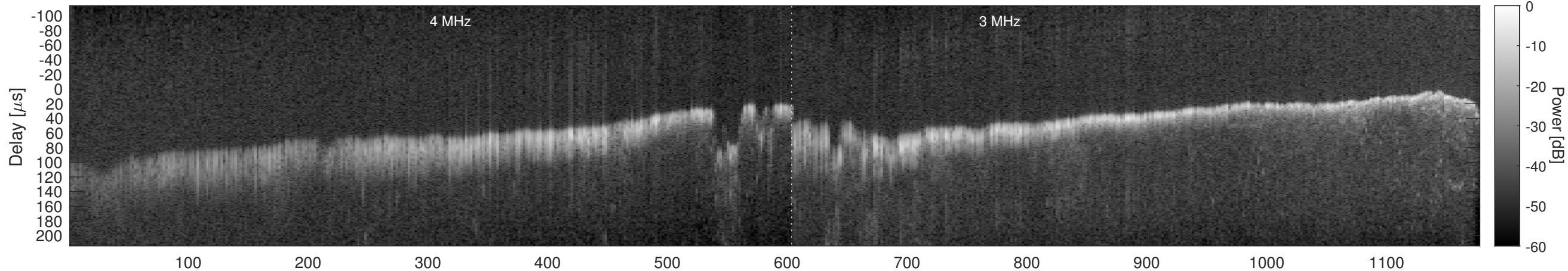
Orbit 18702, Window, Channel 2, Chapman
