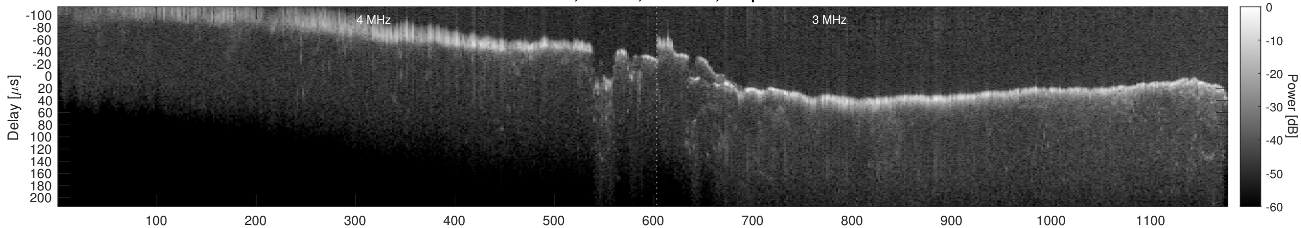
Orbit 18702, Window, Channel 2, Optimized
