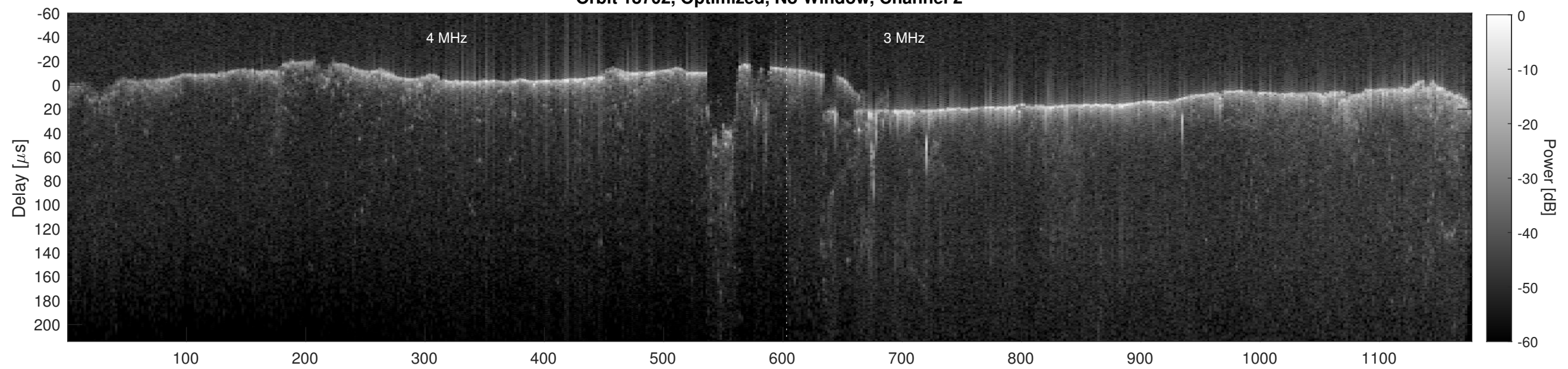
Orbit 18702, Cluttergram
