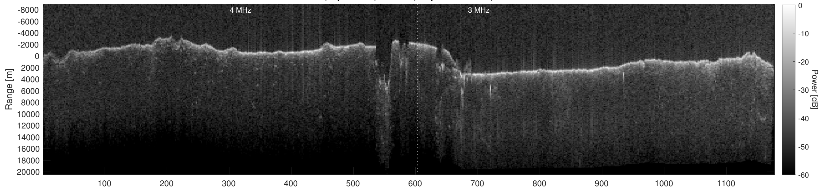
Orbit 18702, Depth-Corrected Cluttergram
