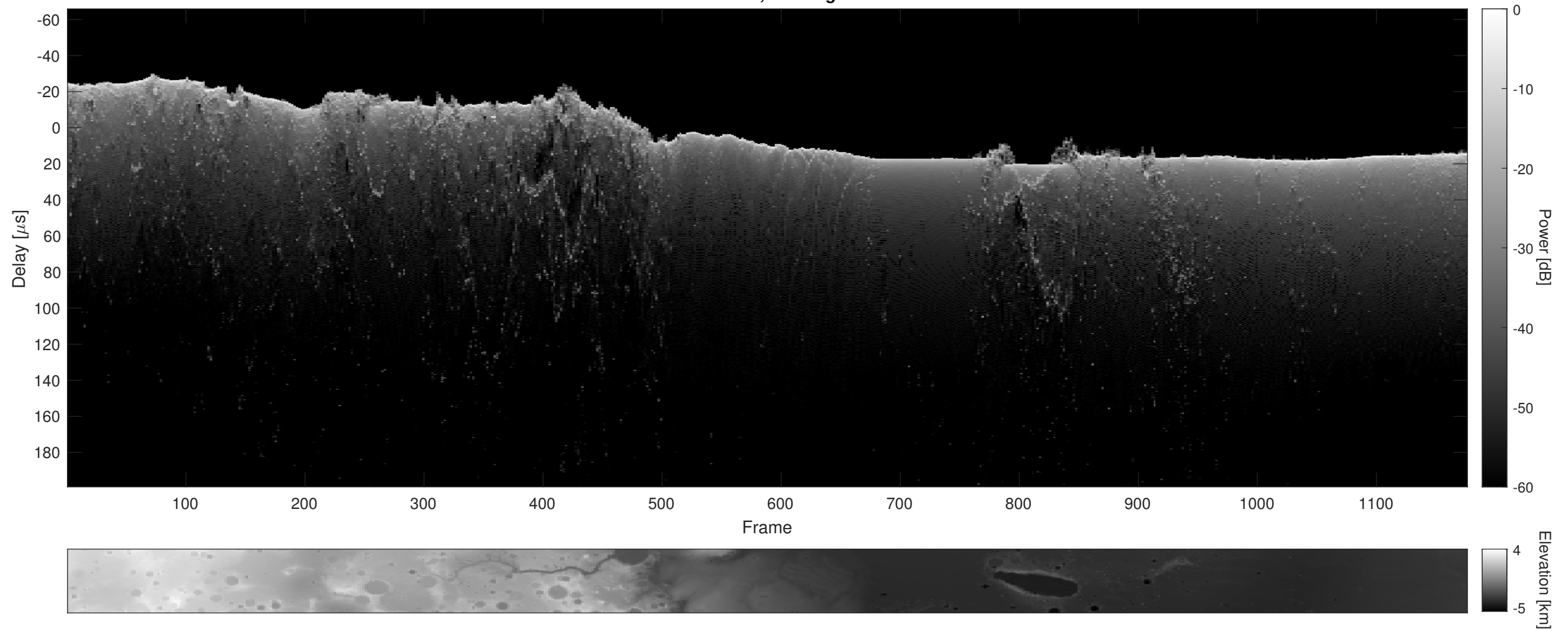
Orbit 18703, Cluttergram
