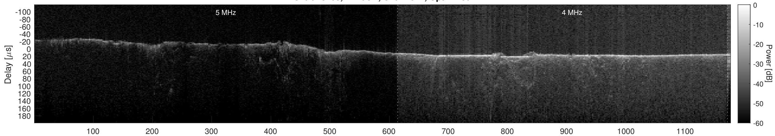
Orbit 18703, Cluttergram
