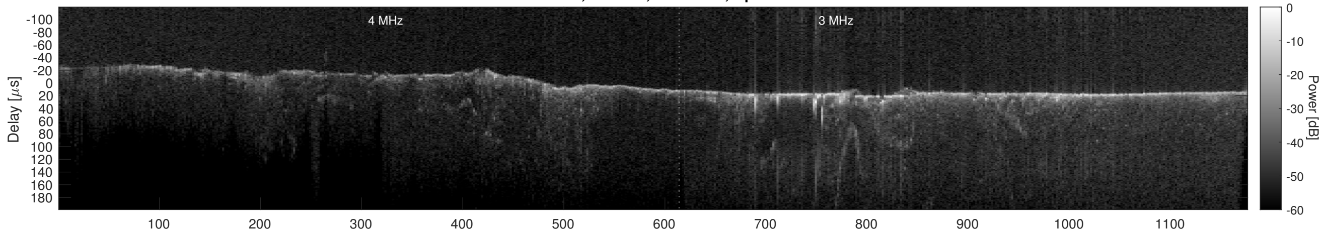
Orbit 18703, Cluttergram
