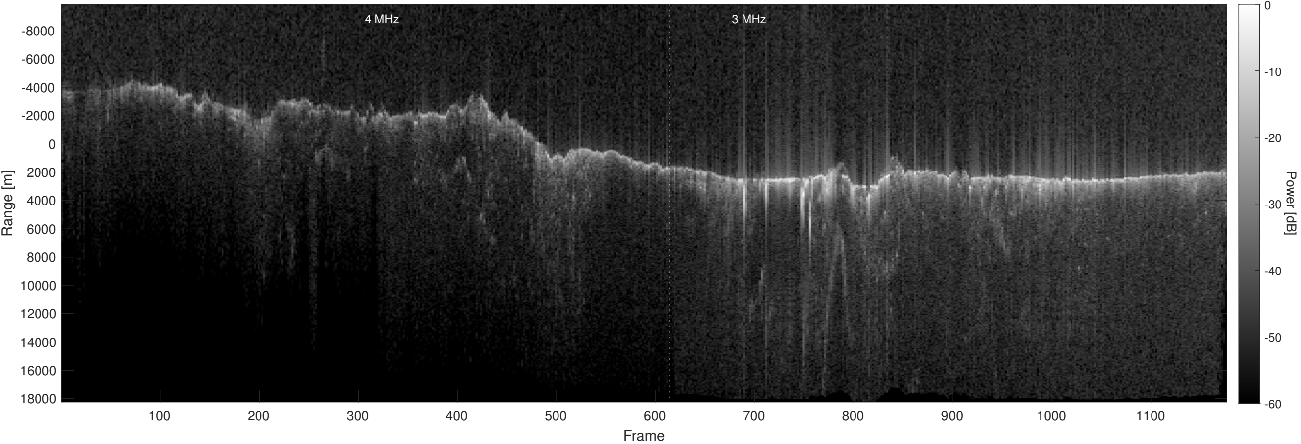
Orbit 18703, Optimized, No Window, Depth-Corrected, Channel 2
