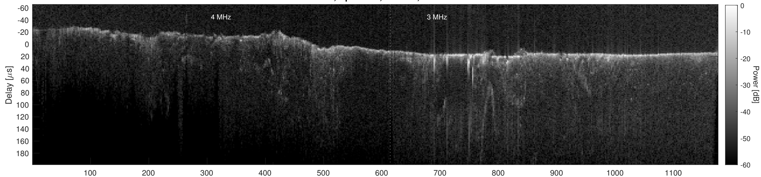
Orbit 18703, Cluttergram
