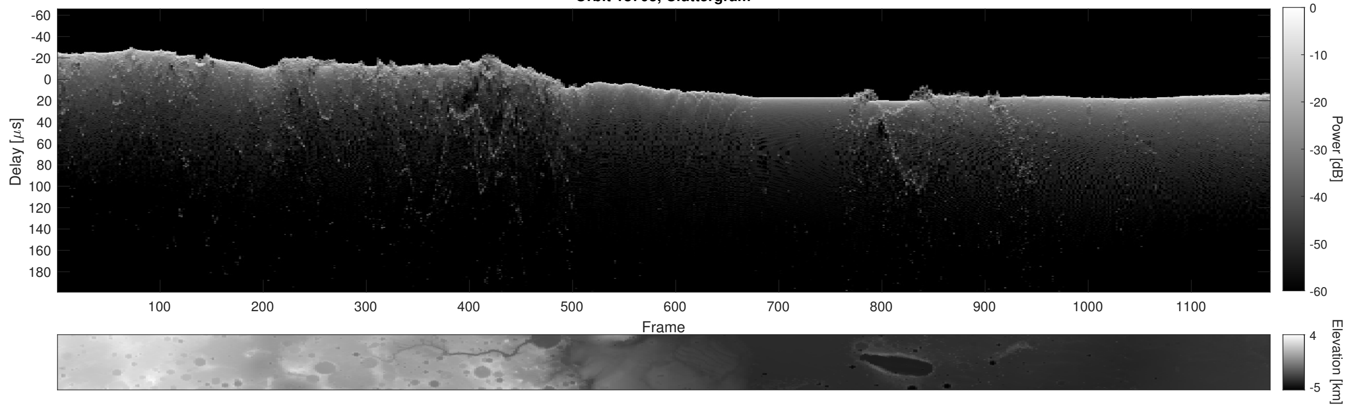
Orbit 18703, Cluttergram
