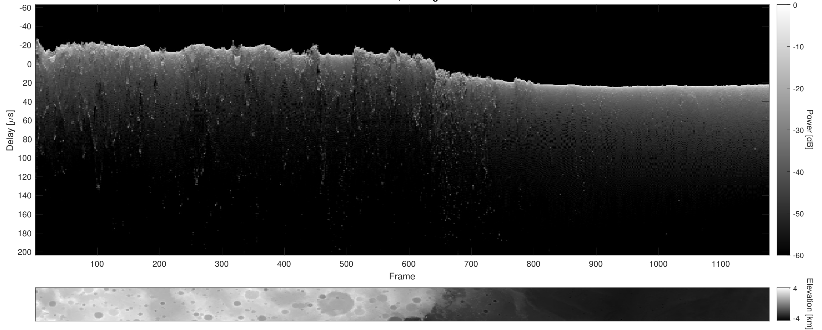
Orbit 18707, Cluttergram
