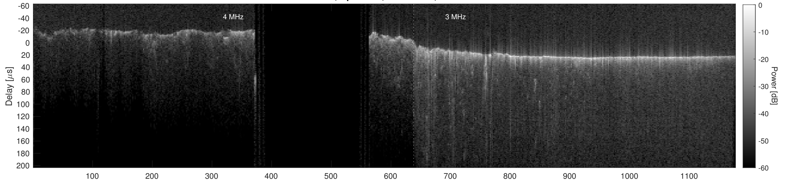
Orbit 18707, Cluttergram
