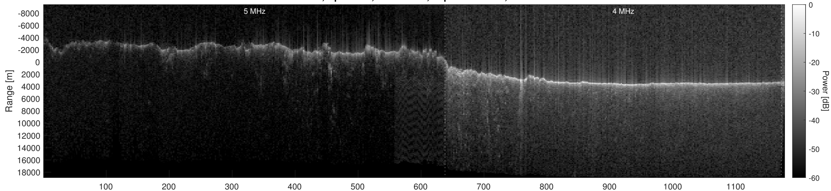
Orbit 18707, Optimized, No Window, Depth-Corrected, Channel 2
