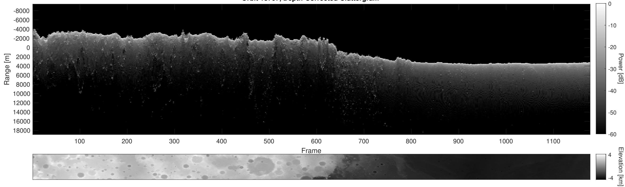
Orbit 18707, Depth-Corrected Cluttergram
