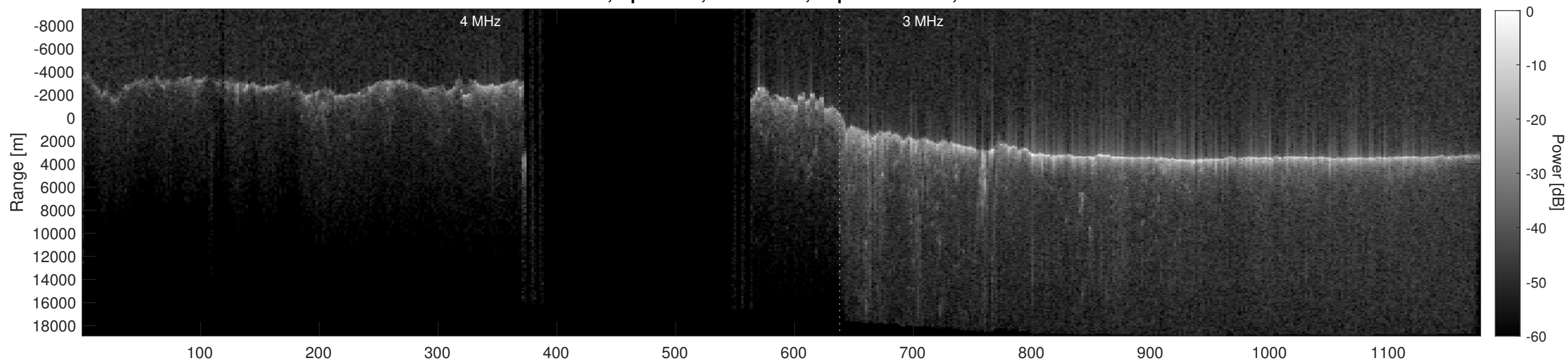
Orbit 18707, Depth-Corrected Cluttergram
