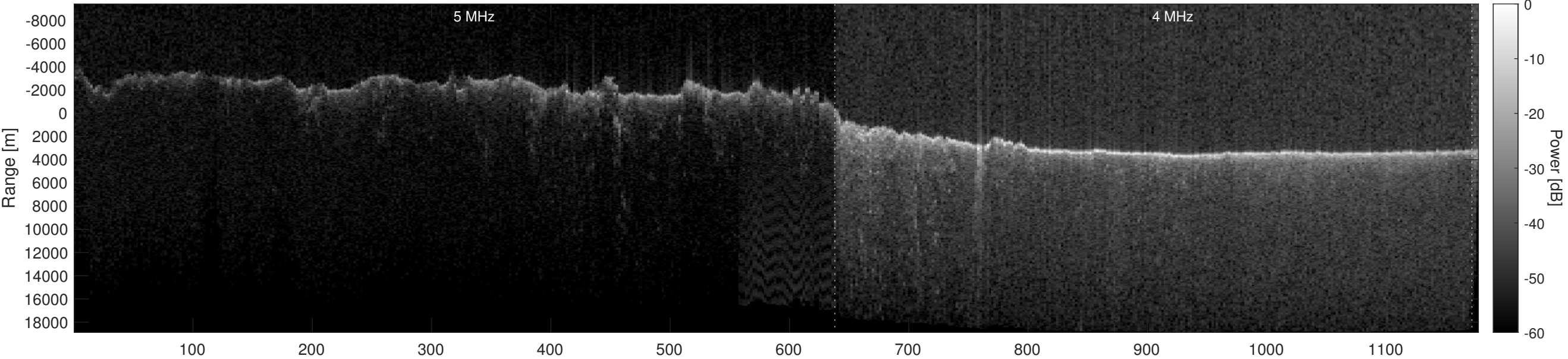
Orbit 18707, Optimized, Window, Depth-Corrected, Channel 2
