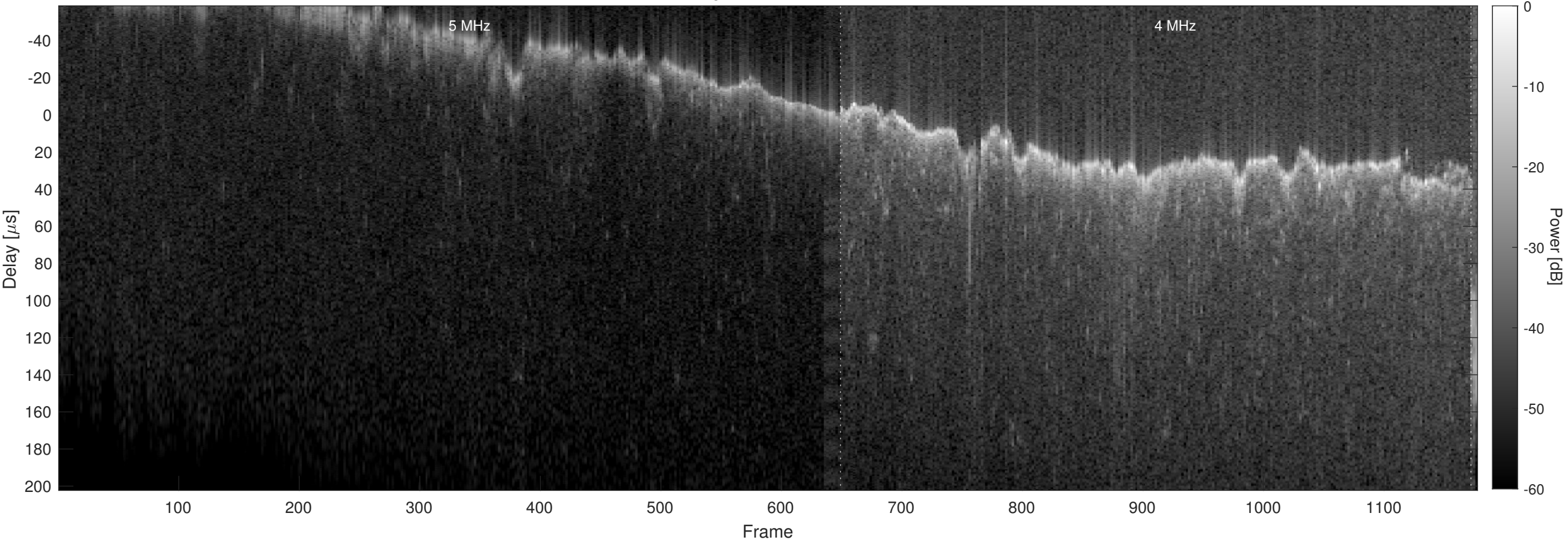
Orbit 18708, Chapman, No Window, Channel 2
