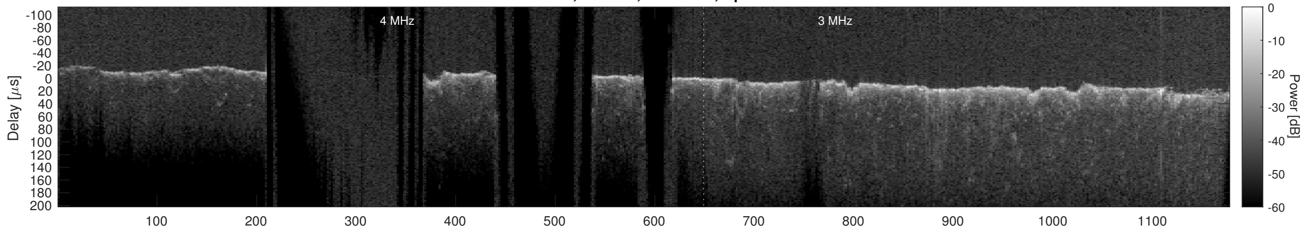
Orbit 18708, Cluttergram
