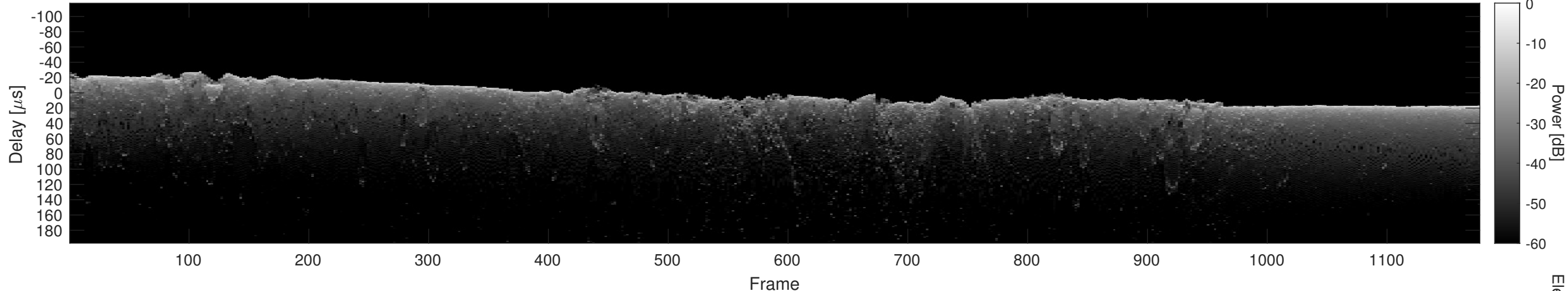
Orbit 18712, Cluttergram
