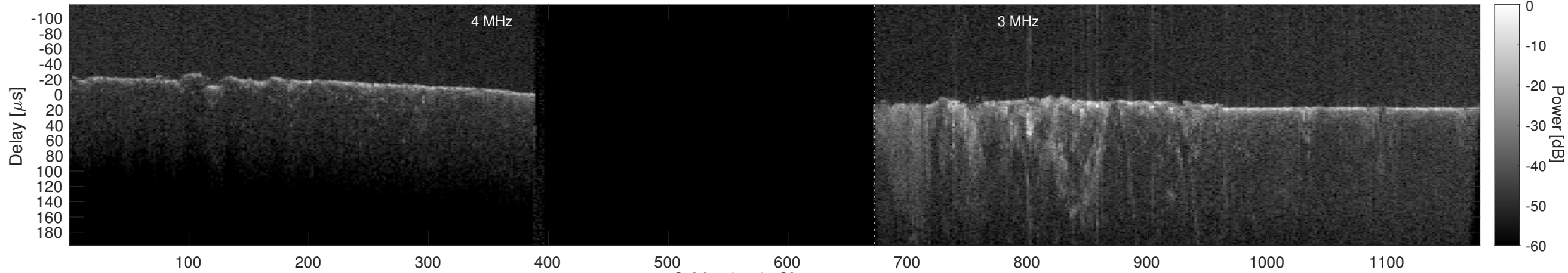
Orbit 18712, Cluttergram
