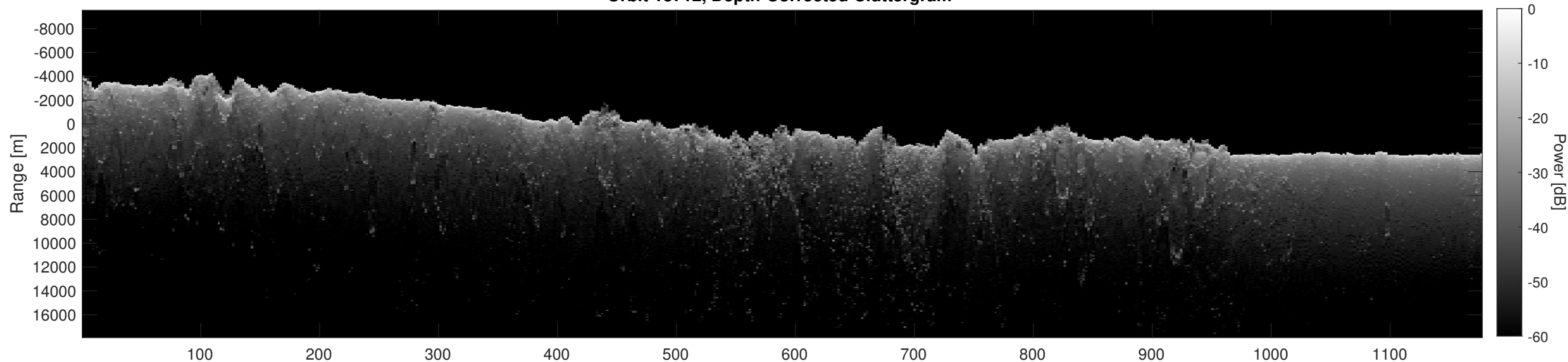
Orbit 18712, Depth-Corrected Cluttergram
