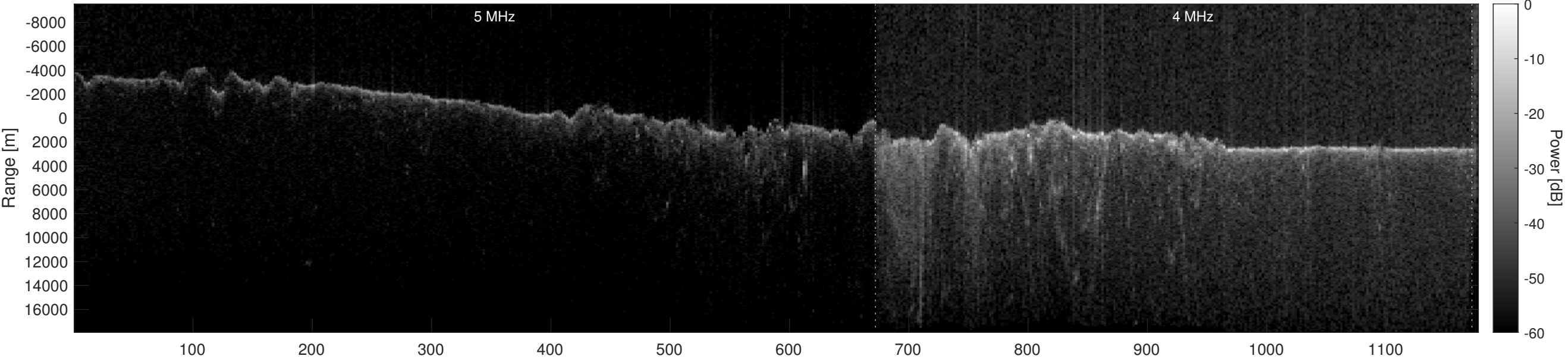
Orbit 18712, Optimized, Window, Depth-Corrected, Channel 2
