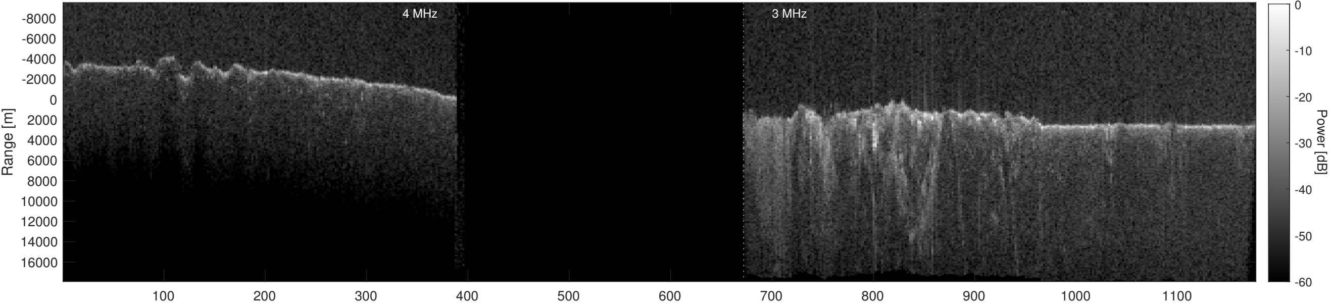
Orbit 18712, Depth-Corrected Cluttergram
