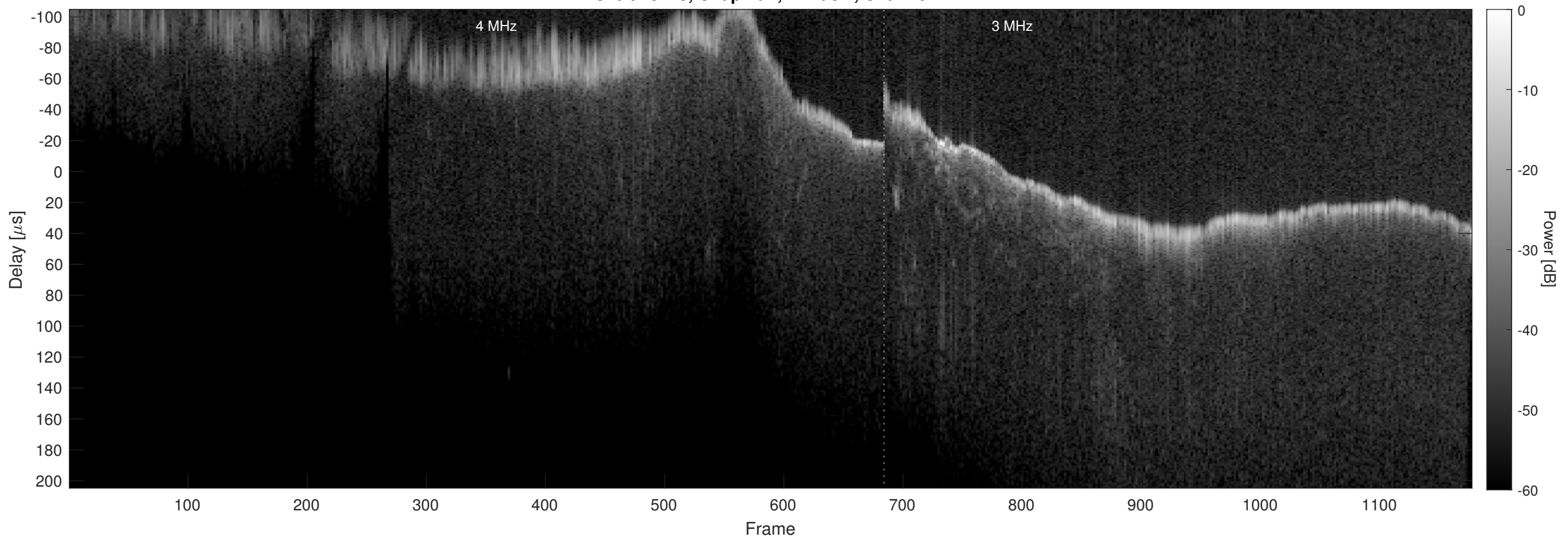
Orbit 18713, Chapman, Window, Channel 2
