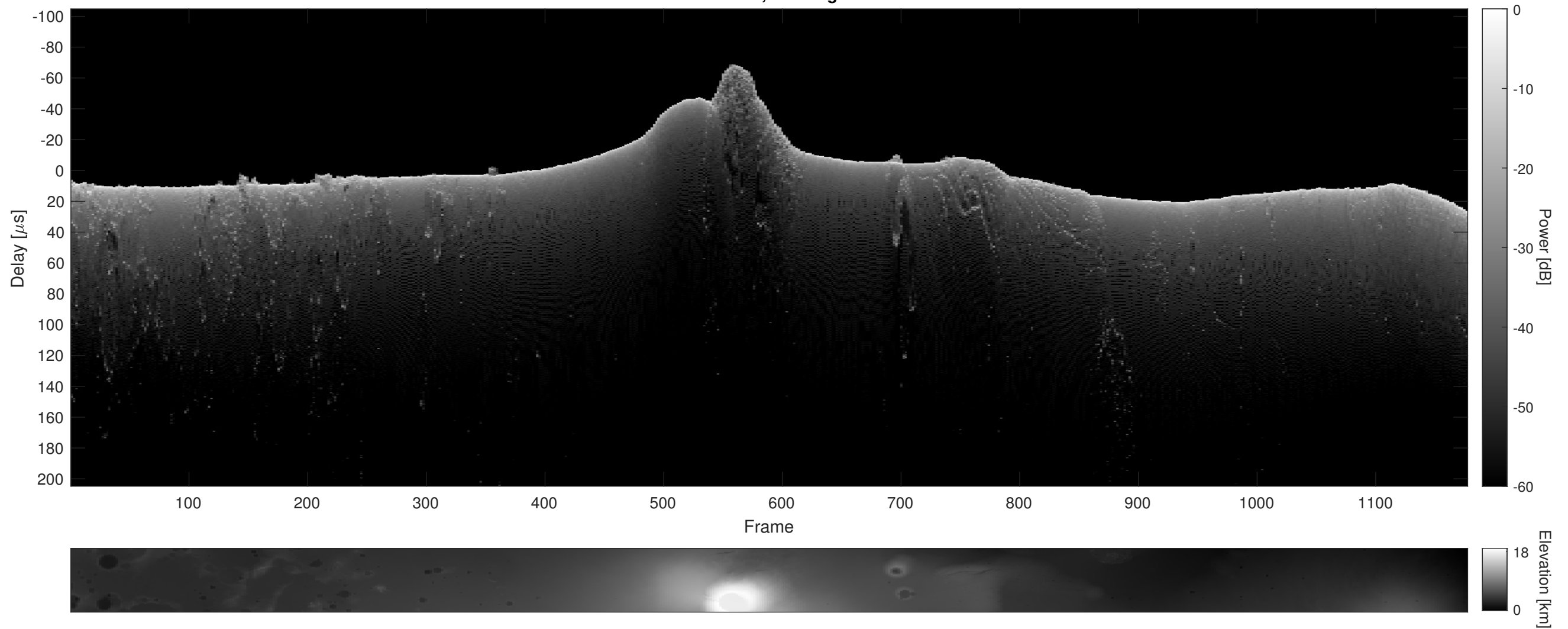
Orbit 18713, Cluttergram
