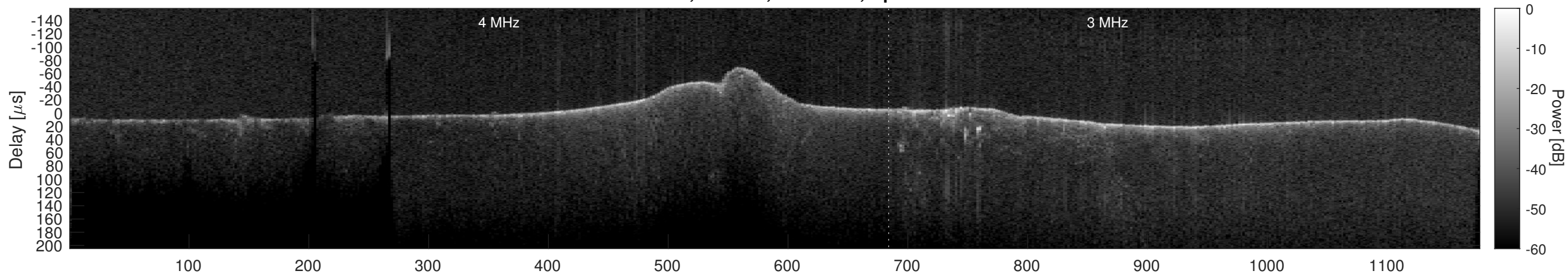
Orbit 18713, Cluttergram
