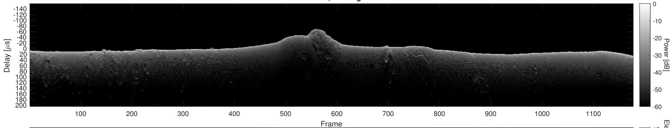
Orbit 18713, Cluttergram
