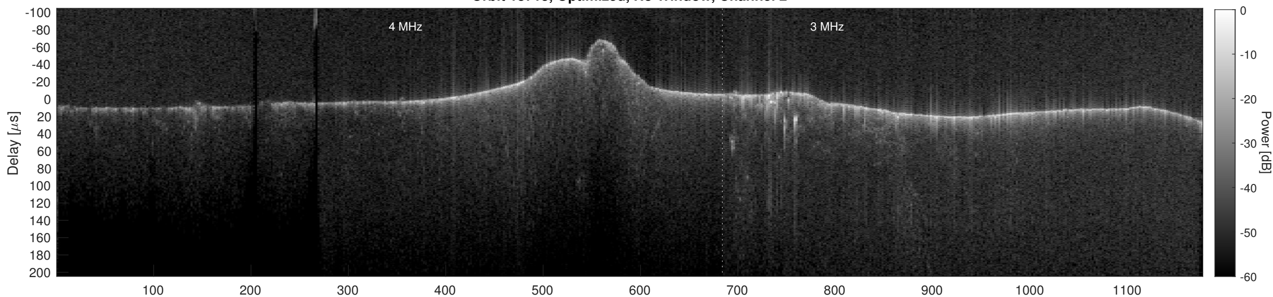
Orbit 18713, Cluttergram
