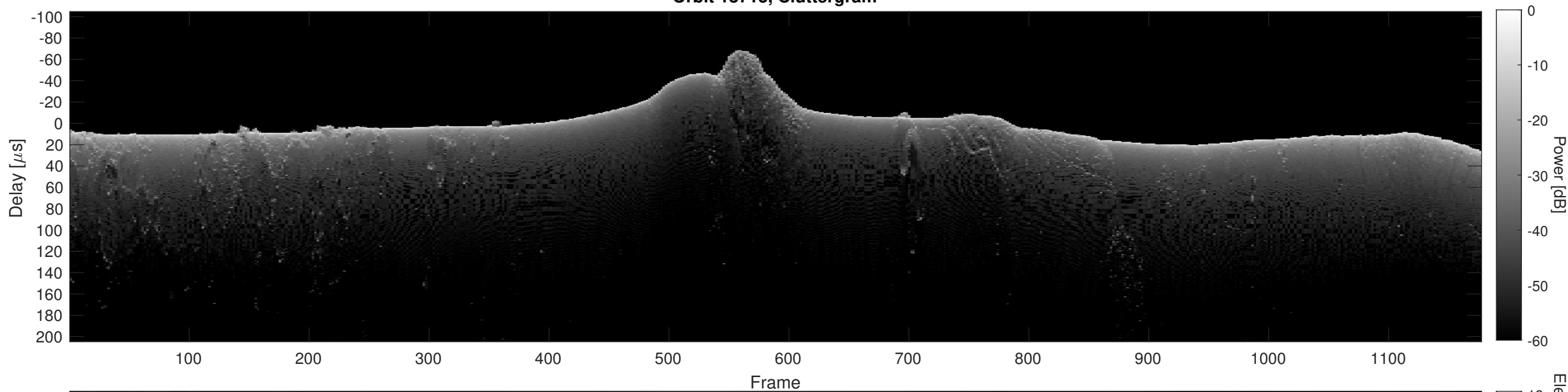
Orbit 18713, Cluttergram
