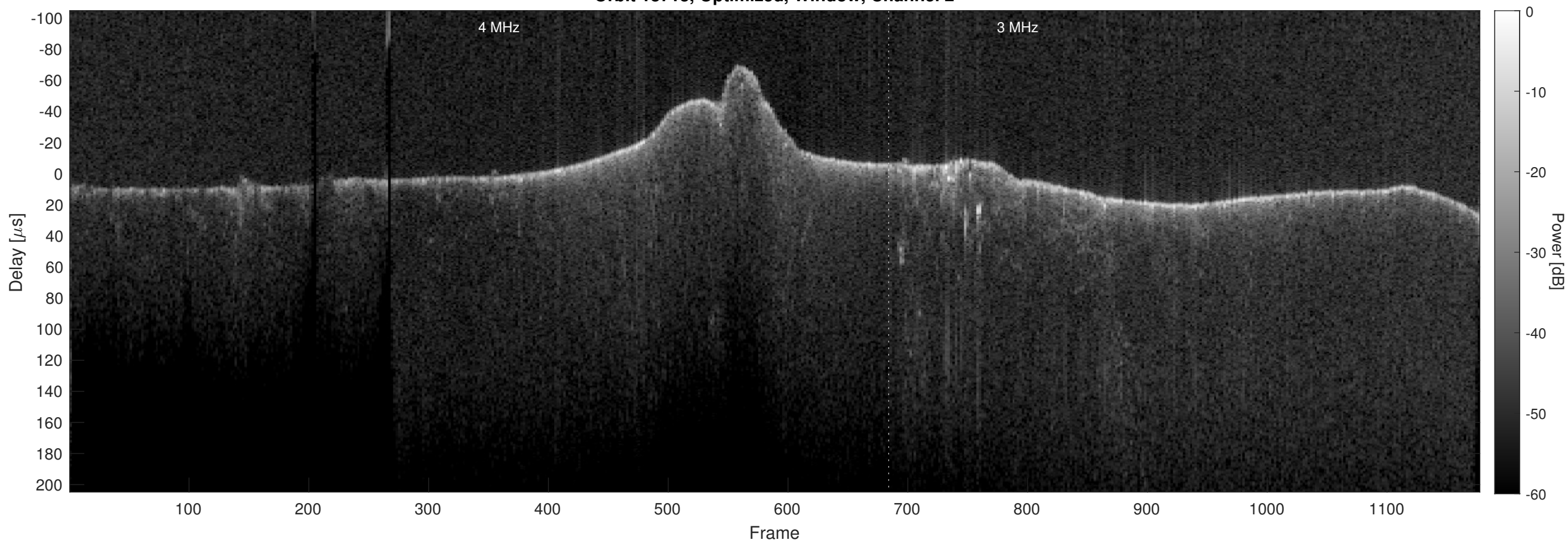
Orbit 18713, Optimized, Window, Channel 2
