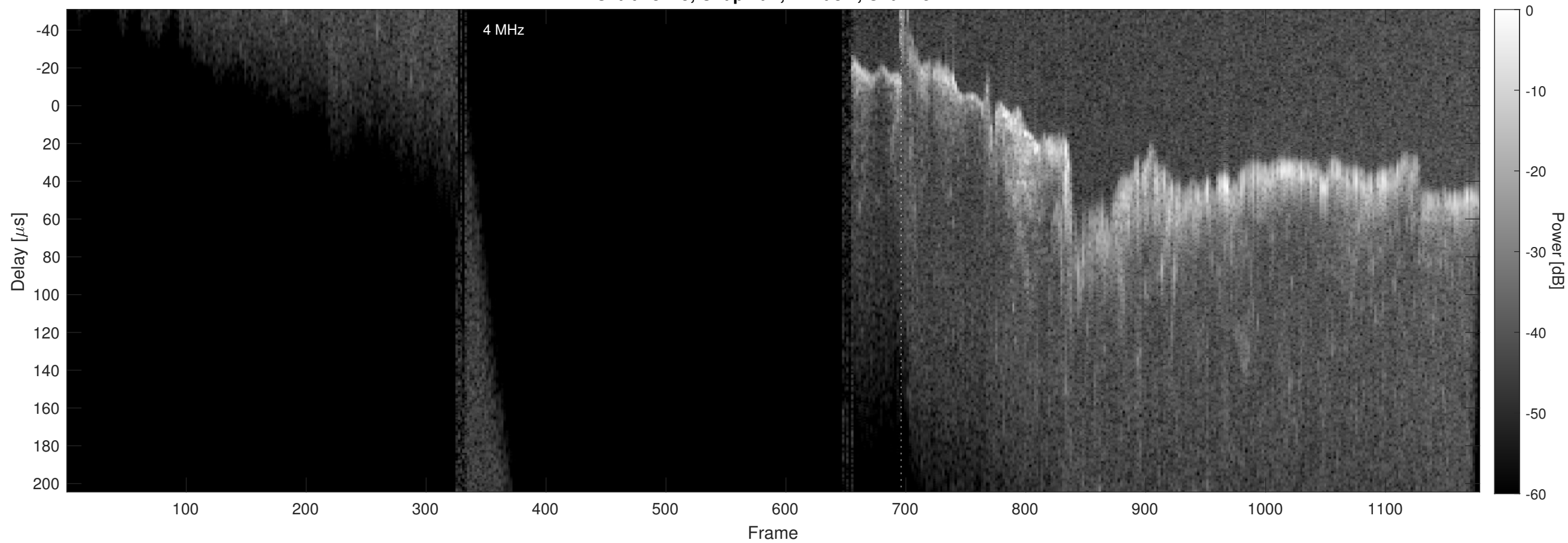
Orbit 18715, Chapman, Window, Channel 2
