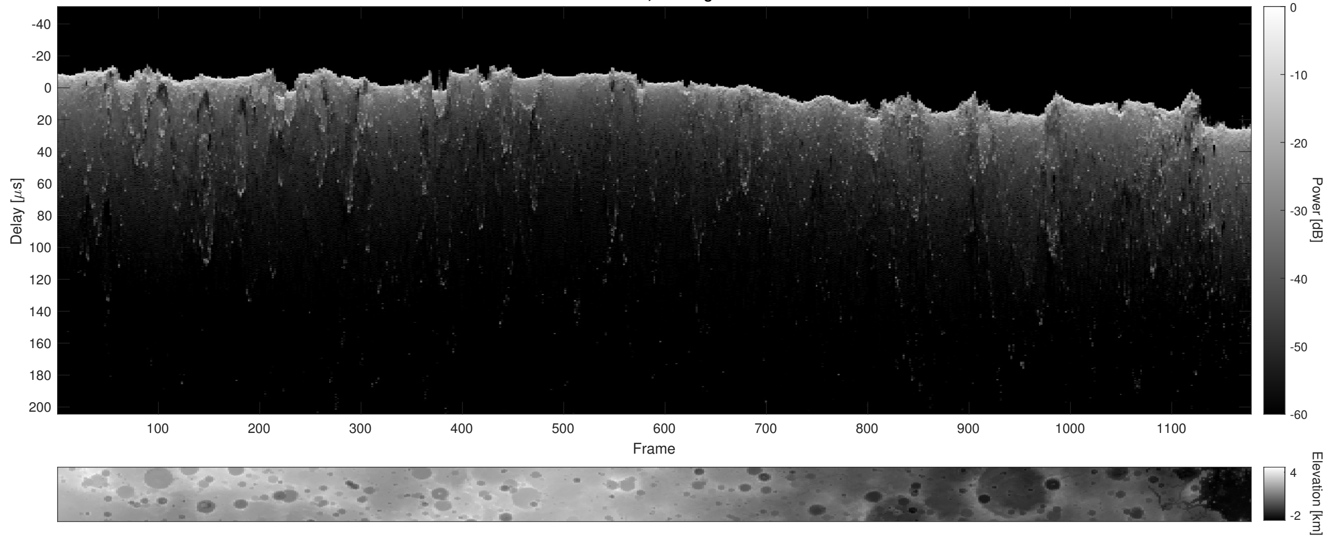
Orbit 18715, Cluttergram
