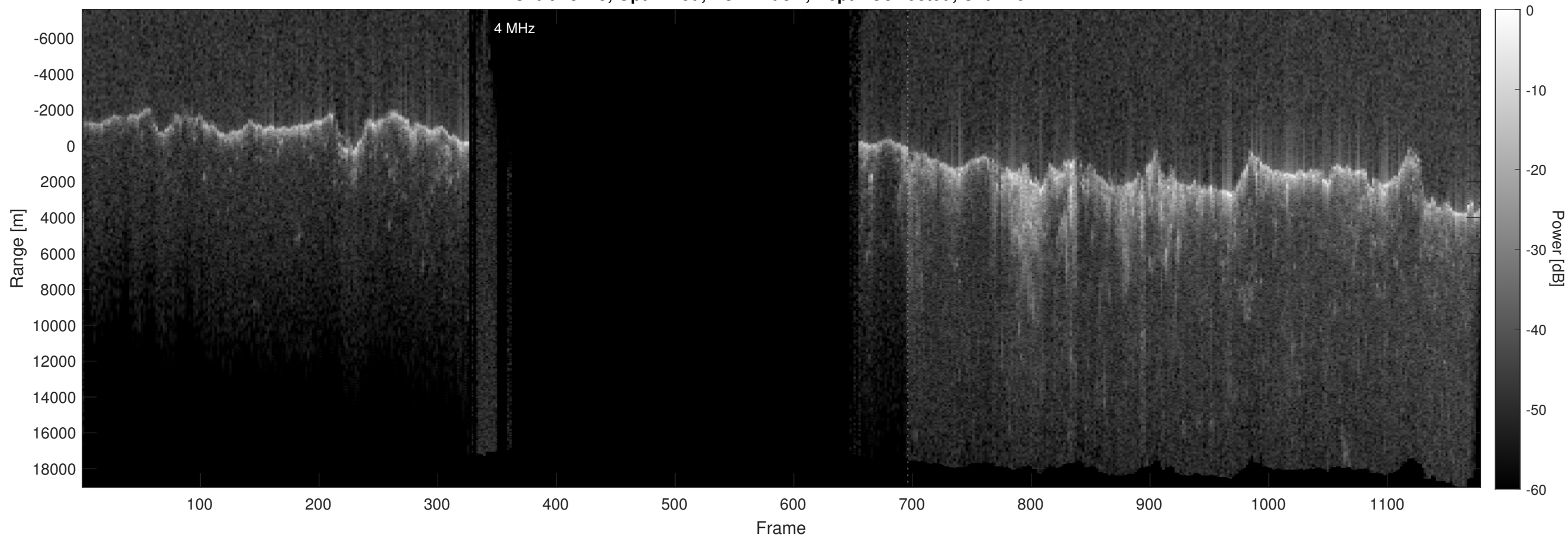
Orbit 18715, Optimized, No Window, Depth-Corrected, Channel 2
