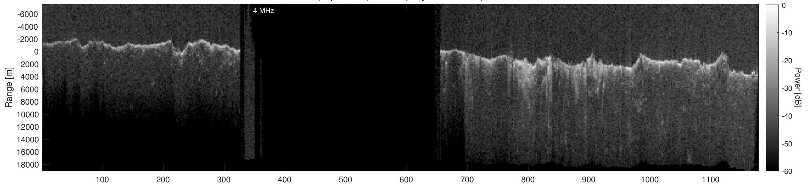
Orbit 18715, Depth-Corrected Cluttergram
