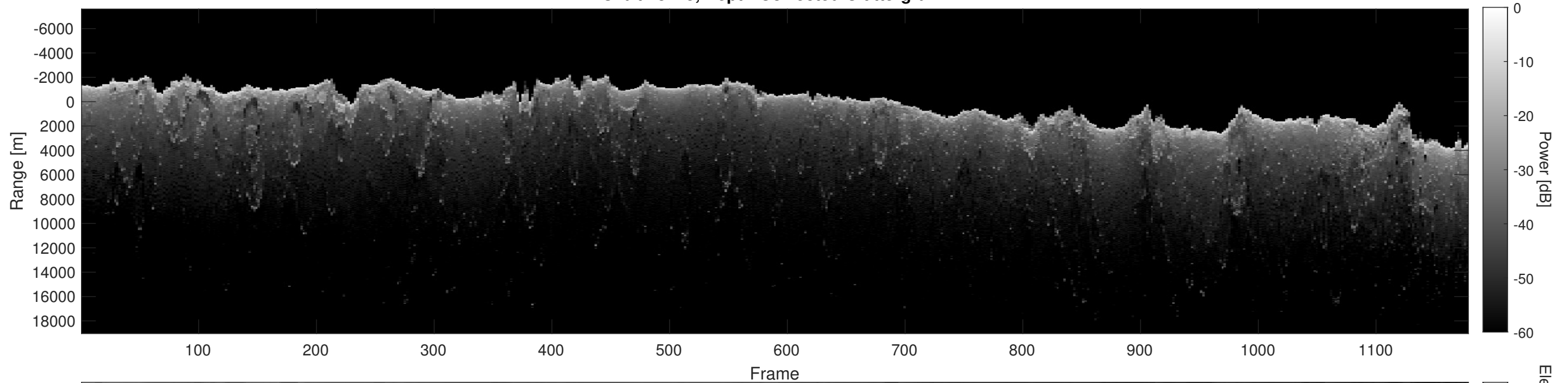
Orbit 18715, Depth-Corrected Cluttergram
