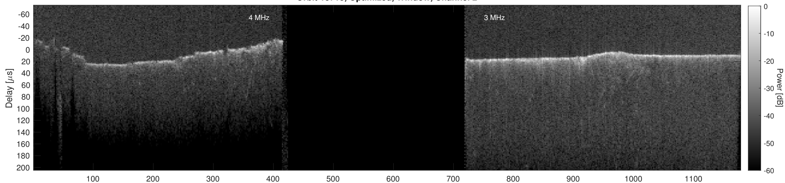
Orbit 18718, Cluttergram
