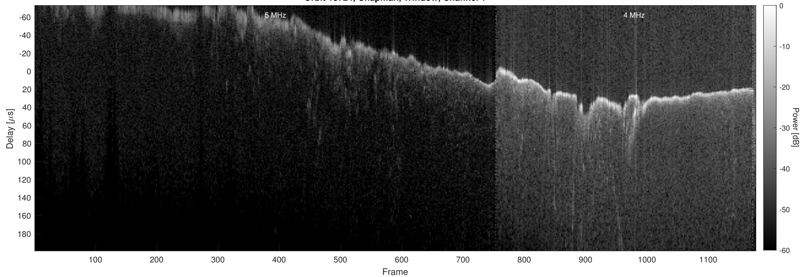
Orbit 18724, Chapman, Window, Channel 2
