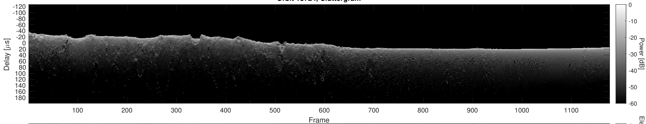
Orbit 18724, Cluttergram
