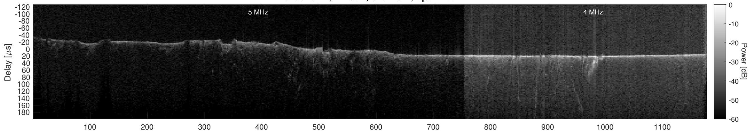
Orbit 18724, Cluttergram
